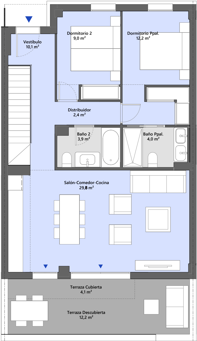
GROUND FLOOR
