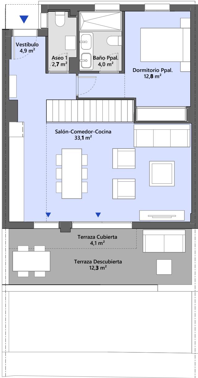
GROUND FLOOR
